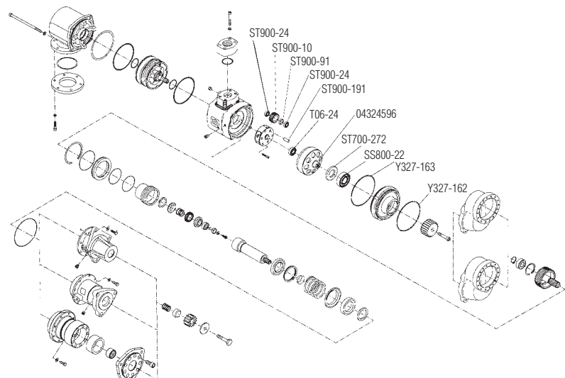
Exploded View of ST900-GK1 Part Location
