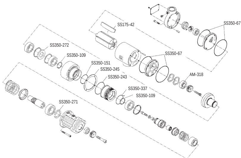
Exploded View of SS175-TK2 Part Location
