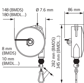
BMDS, BMDLN and BMDLLN
